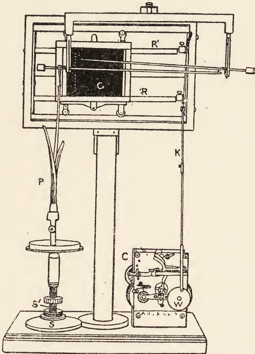
FIG. 17.—The High Magnification Crescograph. P, plant ; C, clockwork for periodic oscillation of recording smoked glass plate (G) ; S S', micrometer screws ; K, crank ; R, eccentric ; W, rotating wheel.
